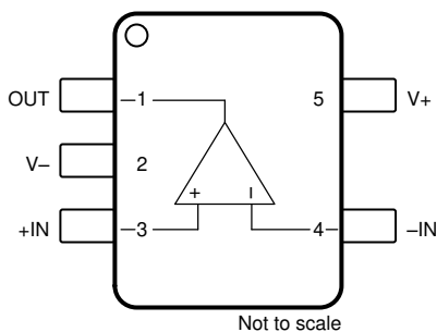
图 5-2. OPA1677 DBV (5-Pin SOT-23) Package, Top View
