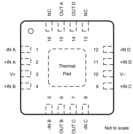
图 5-6. OPA1679 RUM (16-Pin QFN With Exposed Thermal Pad) Package, Top View
