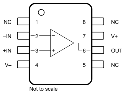
图 5-1. OPA1677 D (8-Pin SOIC) Preview Package, Top View
