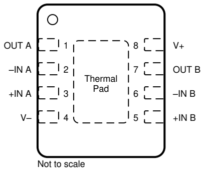
图 5-4. OPA1678 DRG (8-Pin SON With Exposed Thermal Pad) Package, Top View
